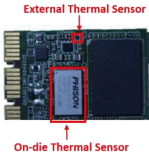
Figure 2-1 Thermal Sensor
