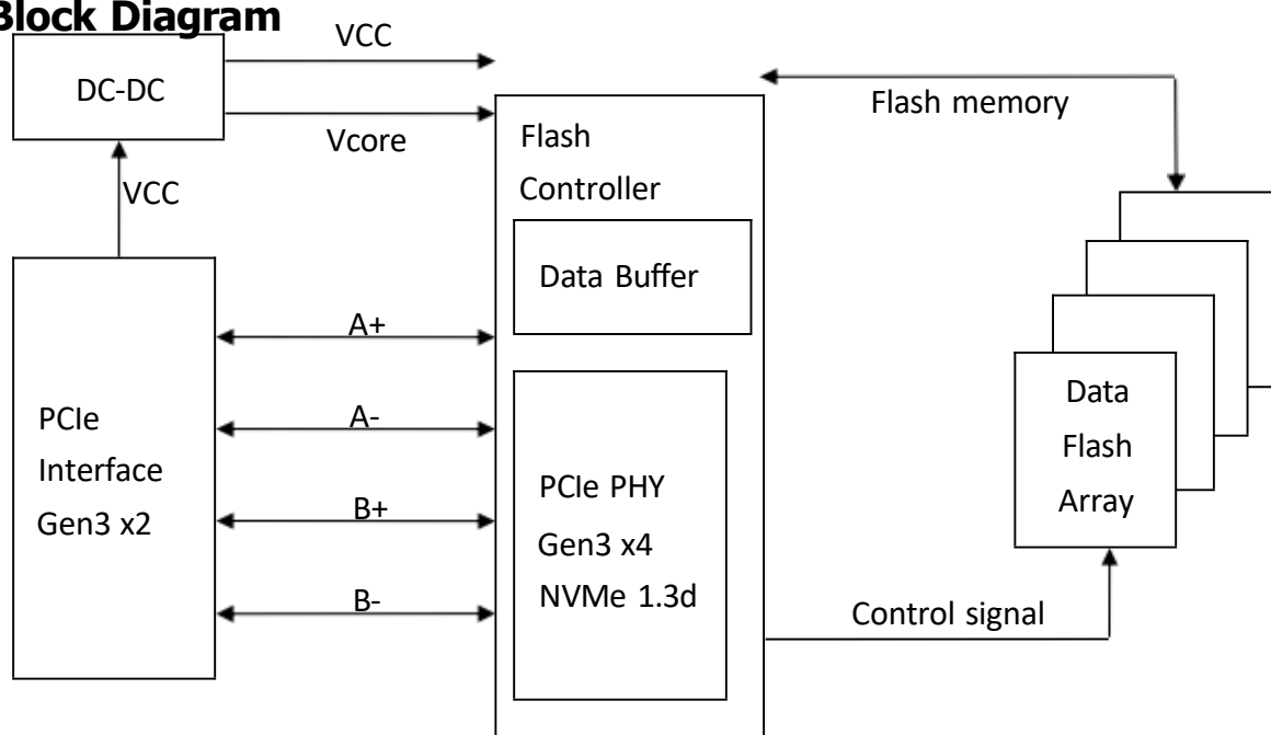
CF Express PCIe SSD Block Diagram
